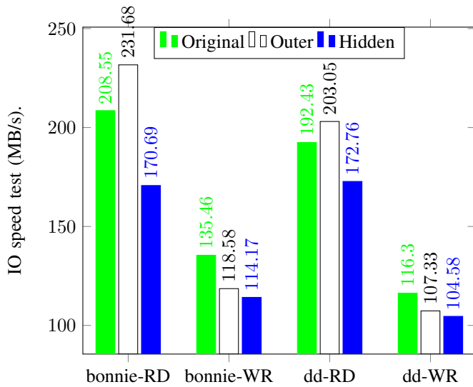
Fig. 6. Bonnie++ Sequential read and write speed (MB/s) and dd read and write speed (MB/s) comparing between outer volume, hidden volume, and original Android FDE. The performance differences between the outer volume and the hidden volume is result from hidden volume has another encryption layer.
